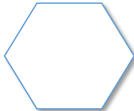
6 sides = Hexagon
